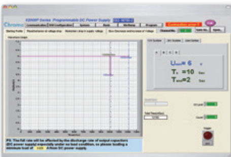
ISO 16750-2 4.5.1 Momentary Drop In Supply Voltage
