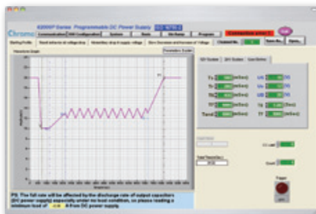
ISO 16750-2 4.5.3 Starting Profile
