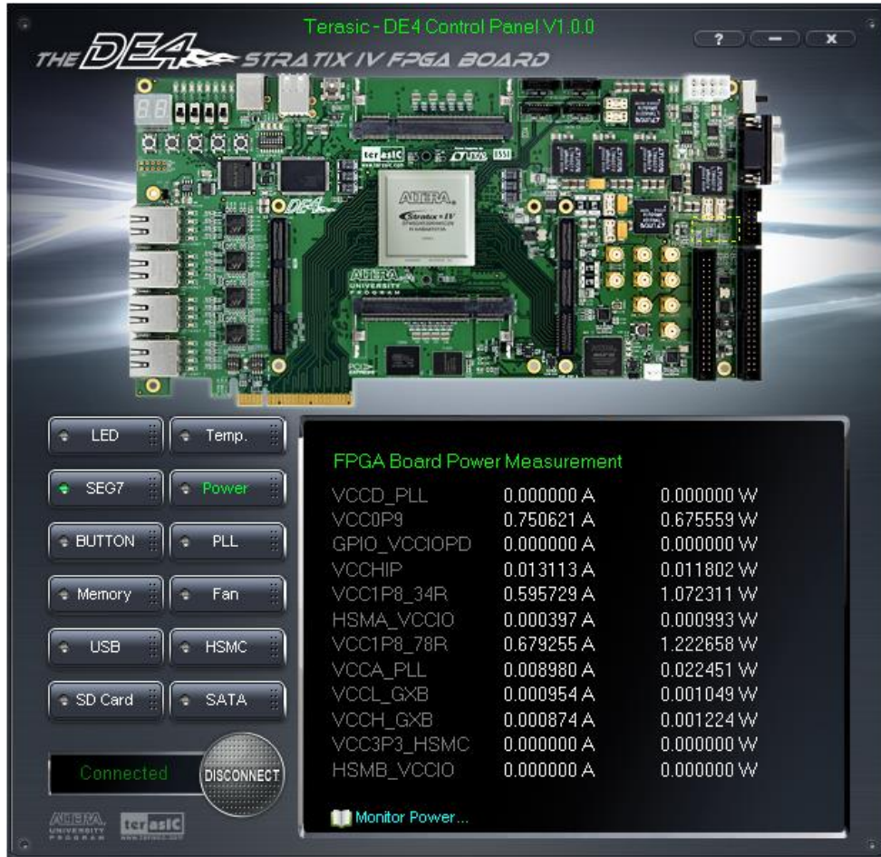
Figure 3–13 Power measurement for the associated power banks of the DE4
