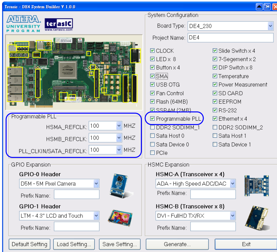
Figure 4-5 External Programmable PLL
